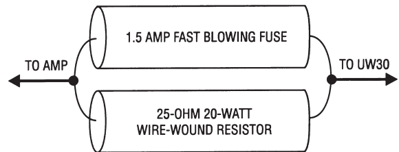
Figure 2 Fuse Recommendation
