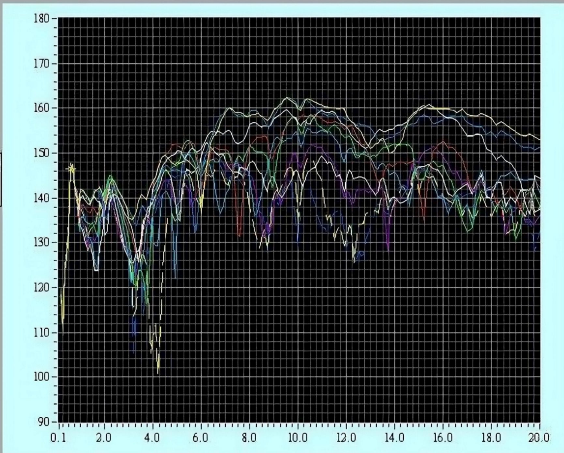
Transmit voltage response vs Frequency
