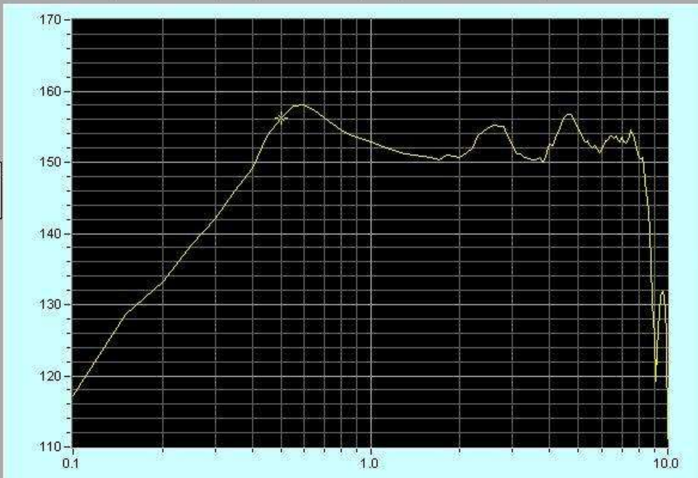
Transmit voltage response vs Frequency
