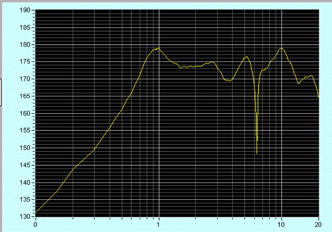
Sound pressure level vs Frequency
