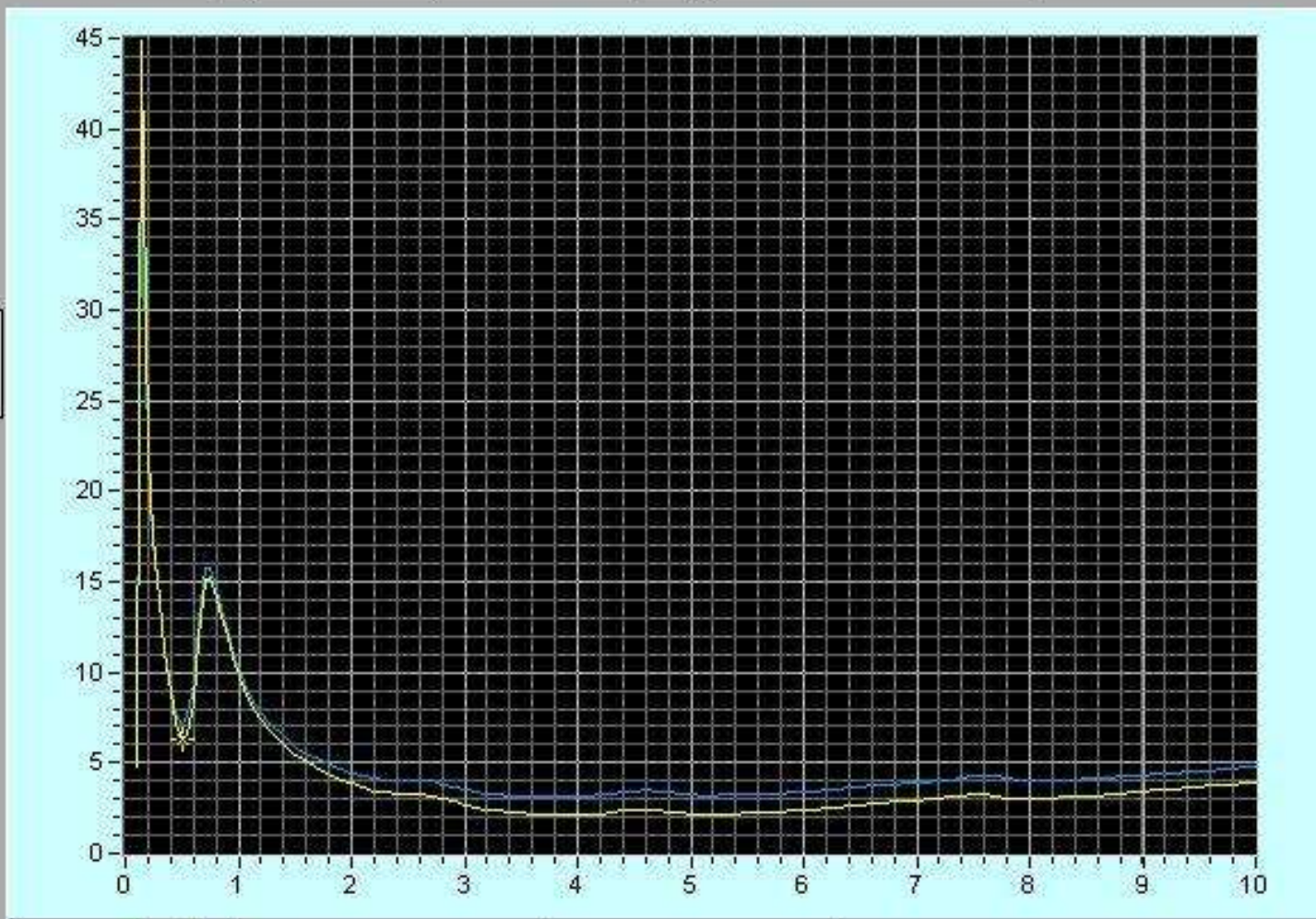
Impedance magnitude vs Frequency
